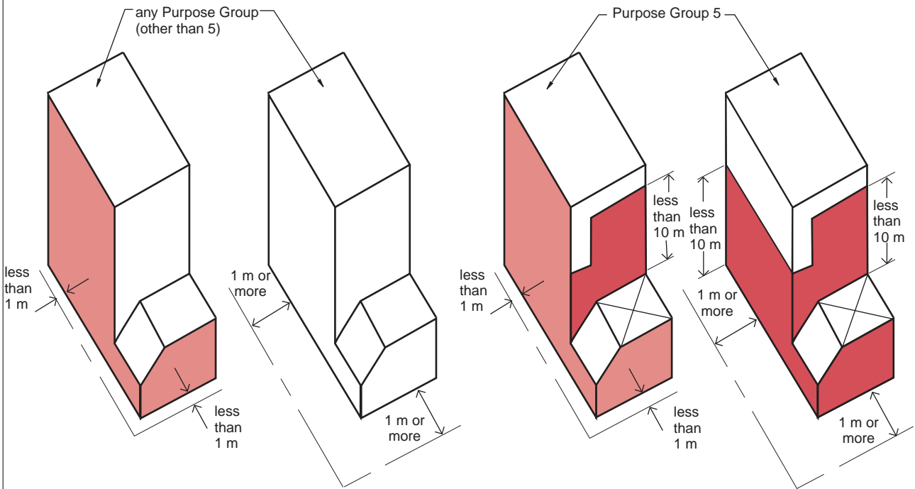
Maximum height of building – less than 18 m
