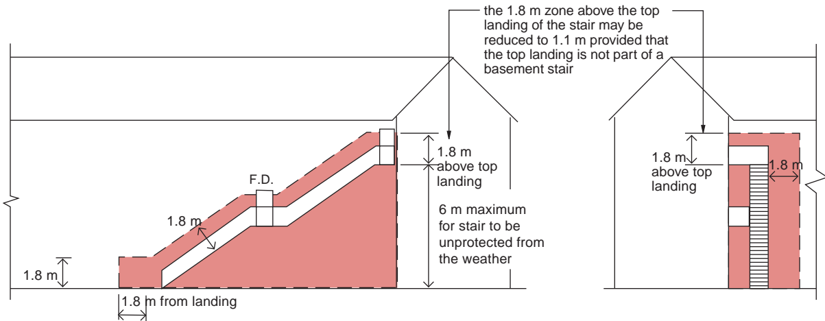
elevation b1
