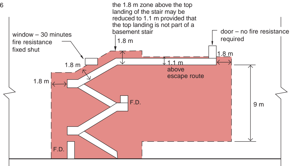
Diagram 2.11 Fire resistance of external walls adjacent to external escape routes
